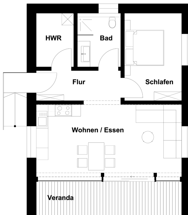
Grundriss eco easy access
